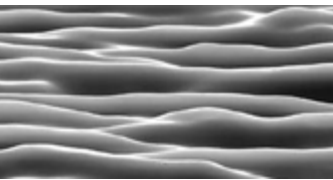
60° x 1° Elliptical LSD SEM Structure 600x
